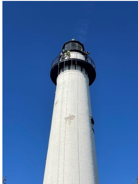
Tower before repairs.
